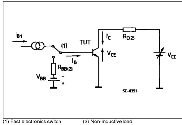
(1) Fast electronics switch (2) Non-inductive load
