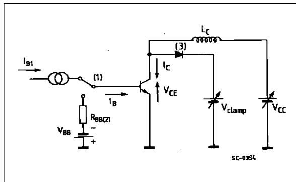
(1) Fast electronic switch (2) Non-inductive load (3) Fast recovery rectifier
